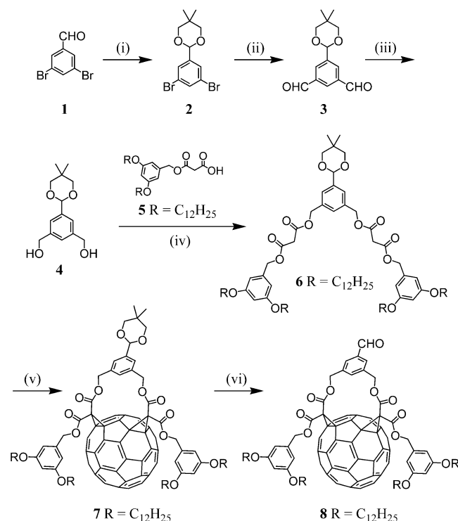
Scheme 1. Reagents and conditions: (i) 2,2-dimethyl-1,3-propanediol, C 6 H 6 , p TosOH cat., \Delta , Dean-Stark trap (97%); (ii) t BuLi (4 equiv.), THF, -78 to 0 °C, then DMF, -78 to 0 °C, then aq. 2 M HCl (58%); (iii) DIBAL-H, CH 2 Cl 2 , 0 °C (97%); (iv) DCC, DMAP, CH 2 Cl 2 , 0 °C to room temp. (72%); (v) C 60 , DBU, I 2 , toluene, room temp. (48%); (vi) CF 3 CO 2 H, H 2 O, CH 2 Cl 2 , room temp. (93%).
