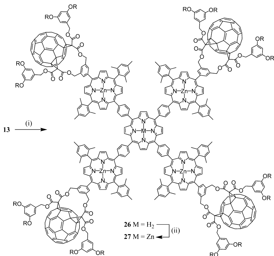
Scheme 5. Reagents and conditions: (i) pyrrole, BF_3 \cdot Et_2O , CHCl_3 (containing 0.75% EtOH ), room temp. then p -chloranil, \Delta (57%); (ii) Zn(OAc)_2 \cdot 2H_2O , CHCl_3/MeOH (9:1), \Delta (82%).
