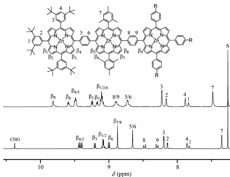
Figure 3. ^1H NMR spectra ( CDCl_3 , 300 MHz) of compounds 23 (bottom) and 25 (top) (solvent peak: S). Unambiguous assignment was achieved on the basis of 2D-COSY and NOESY spectra recorded at room temperature in CDCl_3 .
