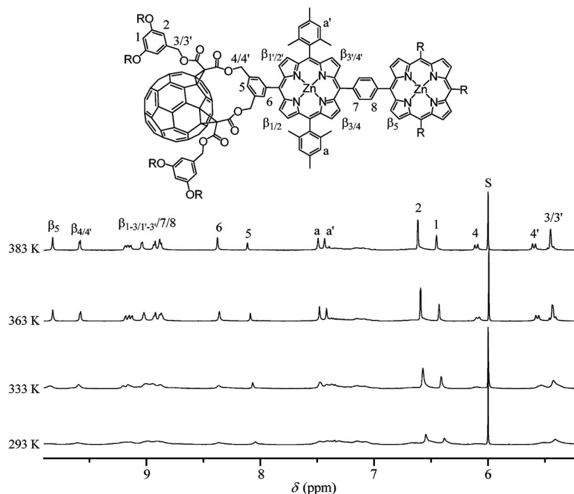
Figure 4. ^1\text{H} NMR spectra (500 MHz) of 27 recorded in \text{CDCl}_2\text{CDCl}_2 at different temperatures (solvent peak: S).
