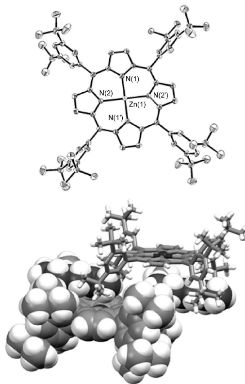
Figure 2. Top: ORTEP plot of the structure of 18 . Thermal ellipsoids are drawn at the 50% probability level. The prime (') characters in the atom labels indicate that these atoms are at equivalent position. Selected bond lengths and bond angles: \text{Zn(1)}\text{--}\text{N(1)} : 2.029(3) \text{ \AA} ; \text{Zn(1)}\text{--}\text{N(2)} : 2.046(3) \text{ \AA} ; \text{N(1)}\text{--}\text{Zn(1)}\text{--}\text{N(2)} : 90.02(11)^\circ ; \text{N(1)}\text{--}\text{Zn(1)}\text{--}\text{N(2')} : 89.98(11)^\circ . Bottom: stacking within the 18 lattice; the co-crystallized hexane molecules are represented in dark grey.
