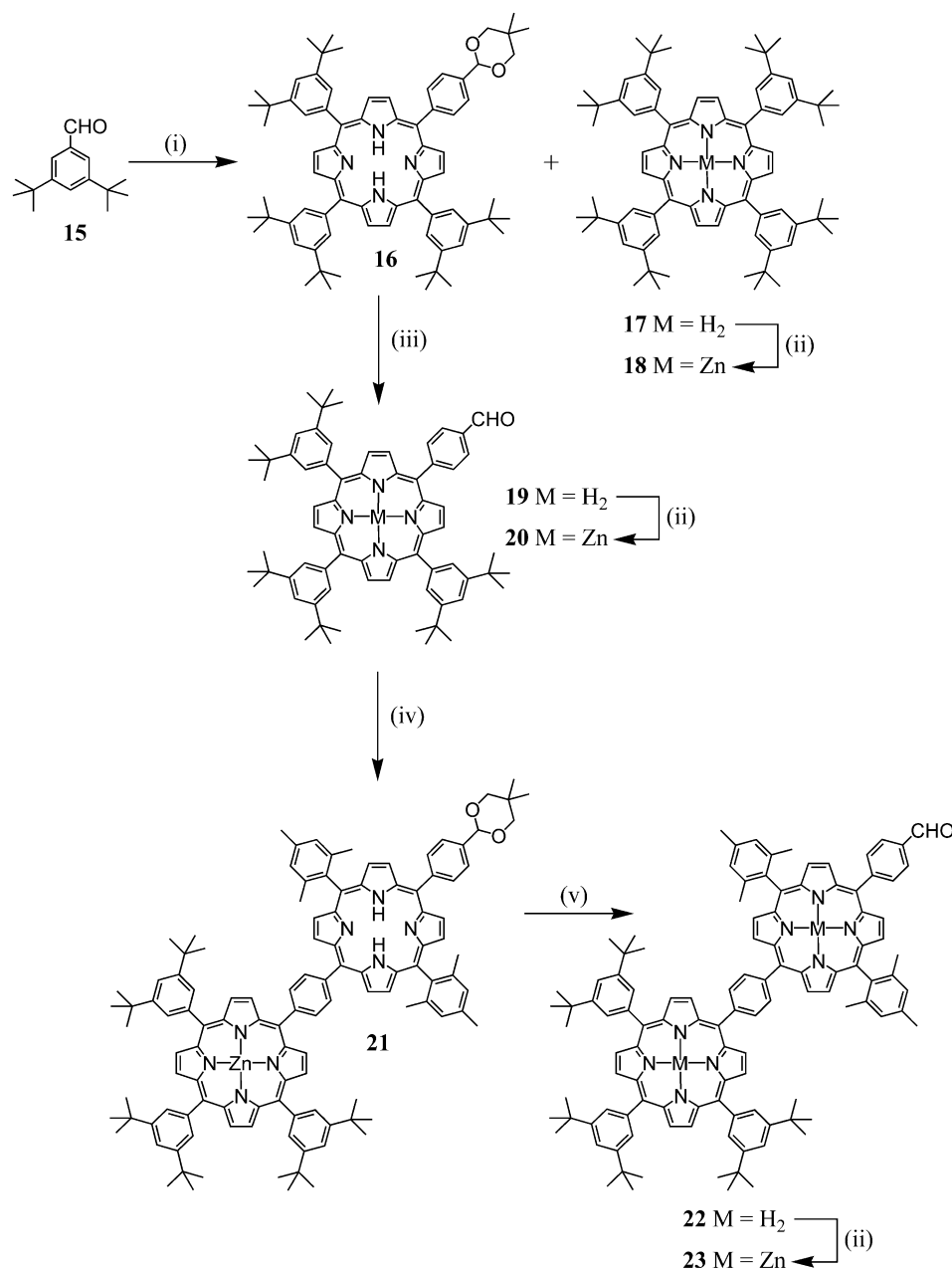
Scheme 3. Reagents and conditions: (i) 9 , pyrrole, BF 3 ·Et 2 O, CHCl 3 (containing 0.75% EtOH), room temp. then p -chloranil, Δ ( 16 : 6% and 17 : 11%); (ii) Zn(OAc) 2 ·2H 2 O, CHCl 3 /MeOH (9:1), Δ ( 18 : 97%; 20 : 92%; 23 : 99%); (iii) CF 3 CO 2 H, H 2 O, CH 2 Cl 2 , room temp. (93%); (iv) 9 , 10 , BF 3 ·Et 2 O, CHCl 3 (containing 0.75% EtOH), room temp. then p -chloranil, Δ (17%); (v) CF 3 CO 2 H, H 2 O, CH 2 Cl 2 , room temp. (93%).
