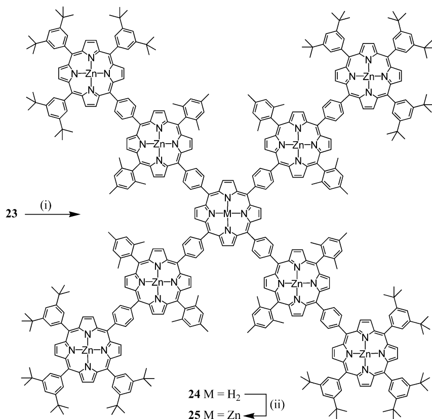
Scheme 4. Reagents and conditions: (i) pyrrole, \text{BF}_3 \cdot \text{Et}_2\text{O} , \text{CHCl}_3 (containing 0.75% EtOH), room temp. then p -chloranil, \Delta (20%); (ii) \text{Zn}(\text{OAc})_2 \cdot 2\text{H}_2\text{O} , \text{CHCl}_3/\text{MeOH} (9:1), \Delta (78%).
